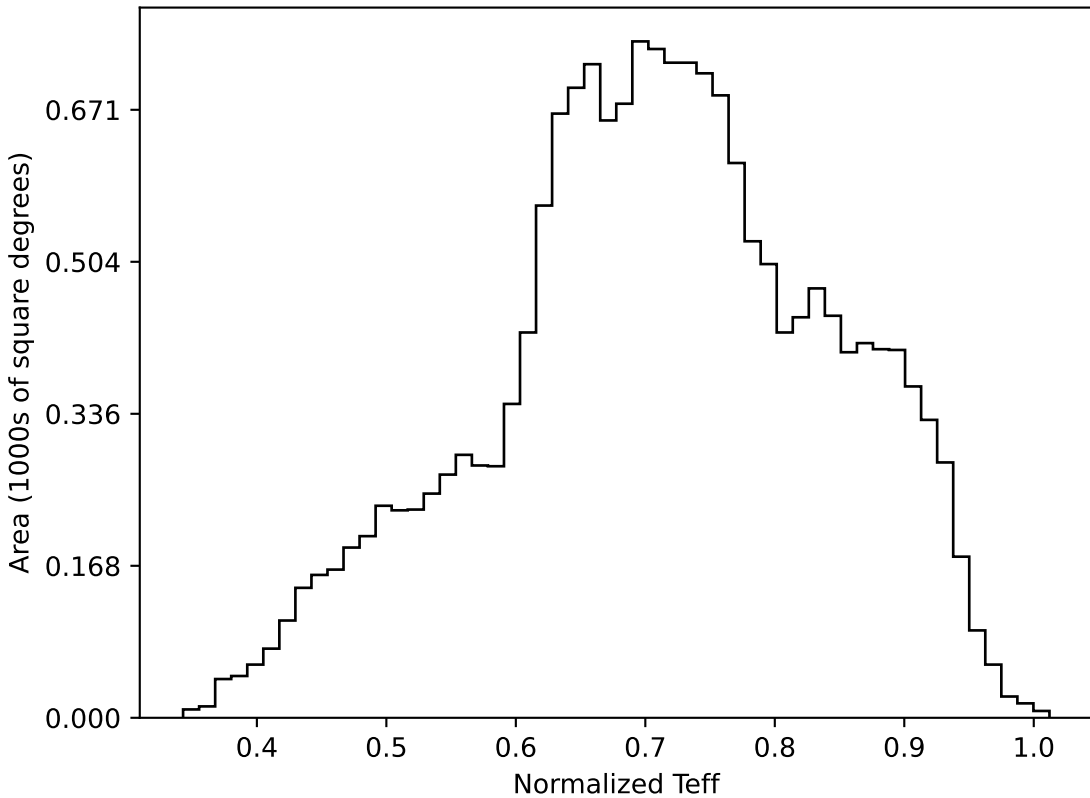
too_100_1v3.4_10yrs WFD all bands: Normalized Teff
