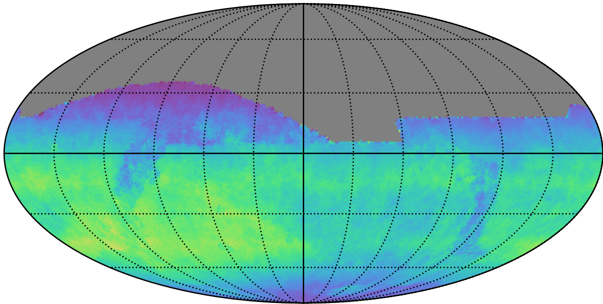
too_100_1v3.4_10yrs All sky z band: Normalized Teff
