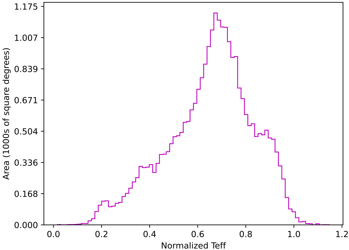
too_100_1v3.4_10yrs All sky z band: Normalized Teff
