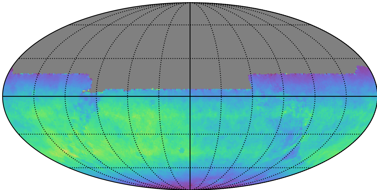
too_100_1v3.4_10yrs All sky y band: Normalized Teff
