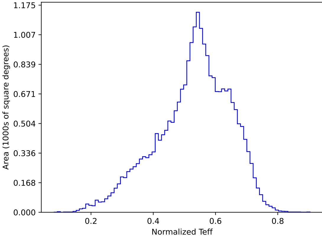
too_100_1v3.4_10yrs All sky y band: Normalized Teff
