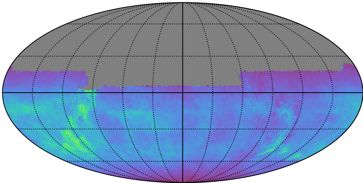
too_100_1v3.4_10yrs All sky u band: Normalized Teff
