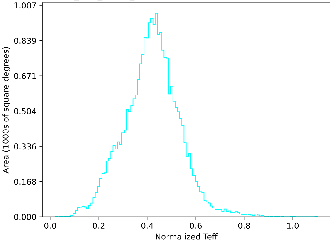
too_100_1v3.4_10yrs All sky u band: Normalized Teff
