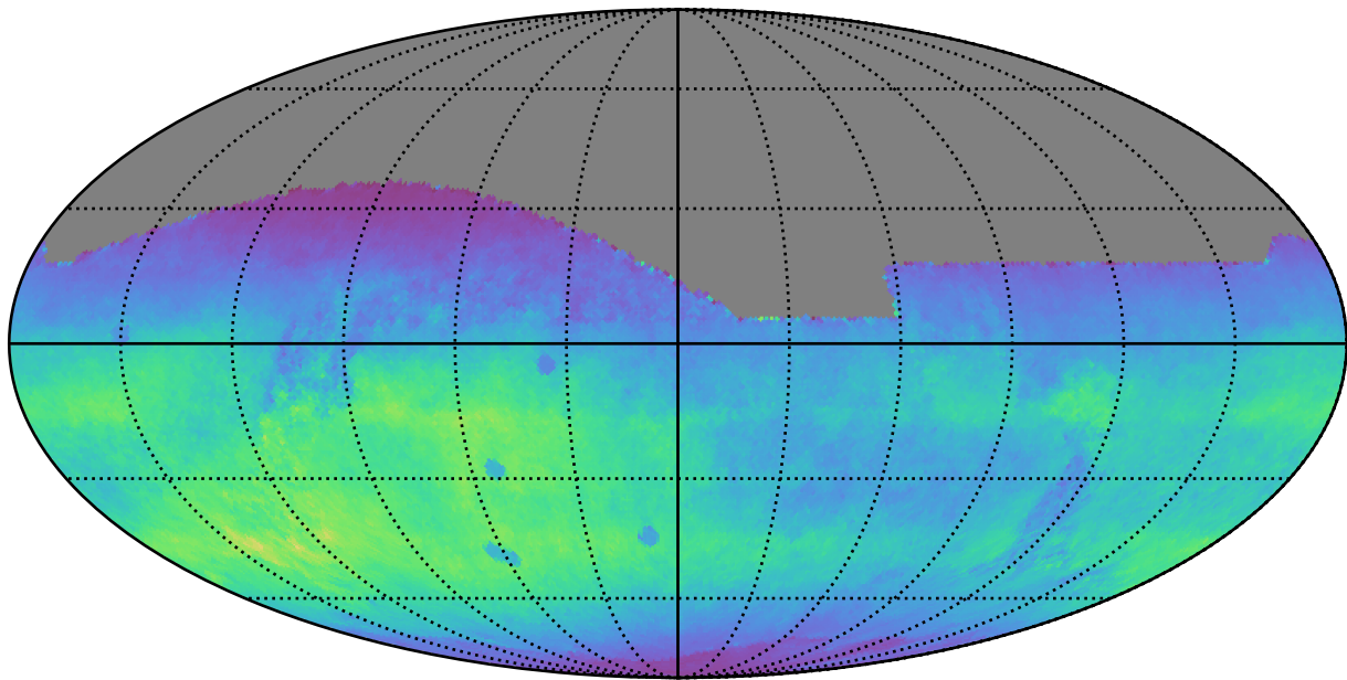
too_100_1v3.4_10yrs All sky r band: Normalized Teff
