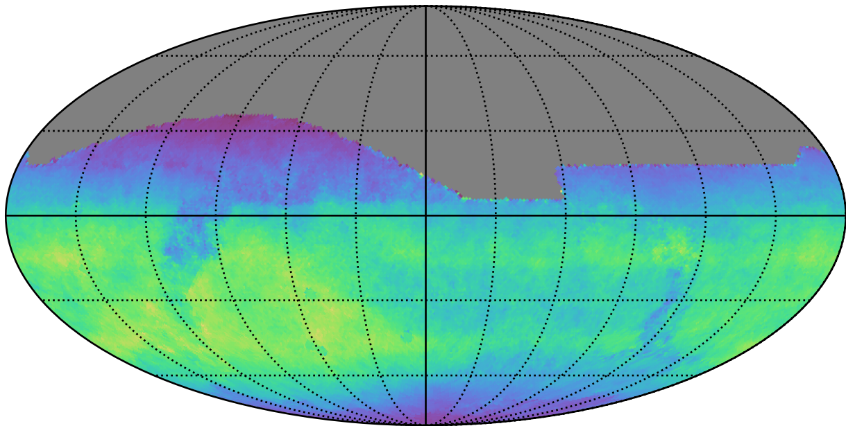
too_100_1v3.4_10yrs All sky i band: Normalized Teff
