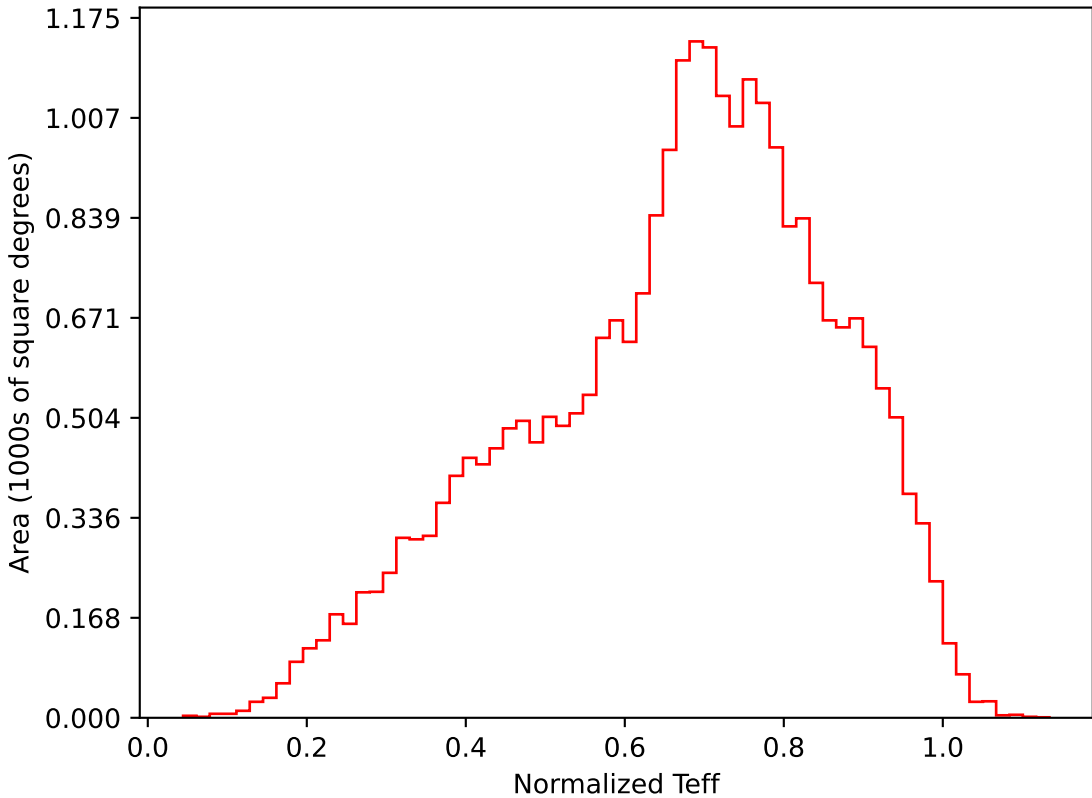
too_100_1v3.4_10yrs All sky i band: Normalized Teff
