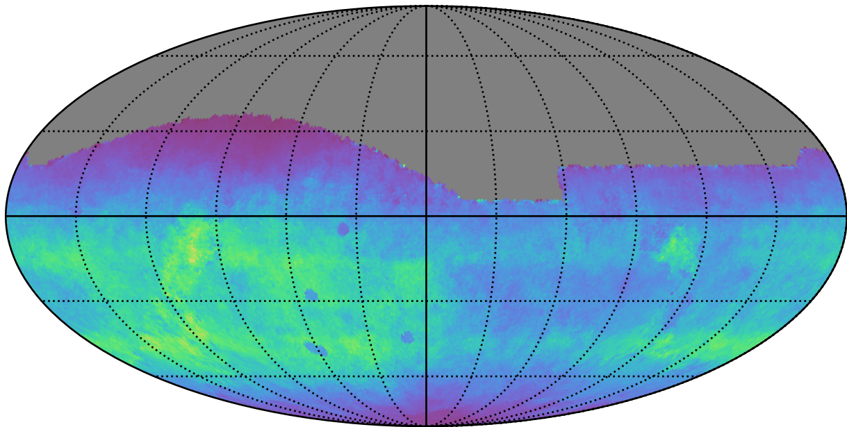
too_100_1v3.4_10yrs All sky g band: Normalized Teff
