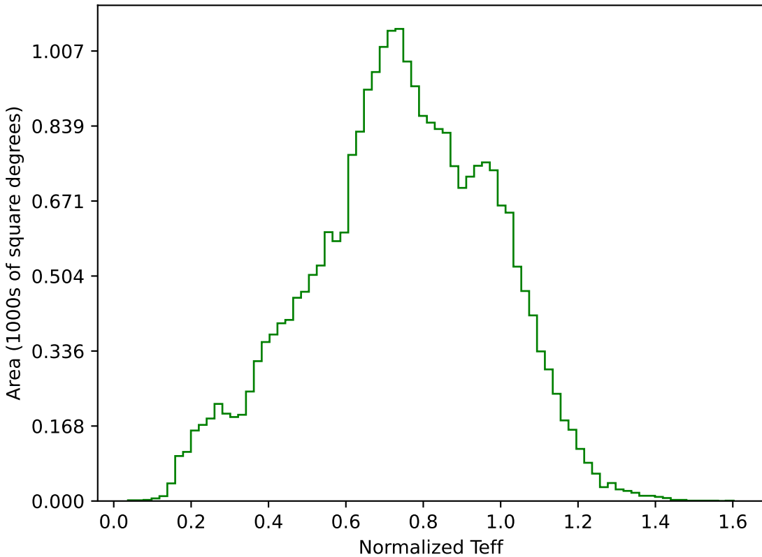
too_100_1v3.4_10yrs All sky g band: Normalized Teff
