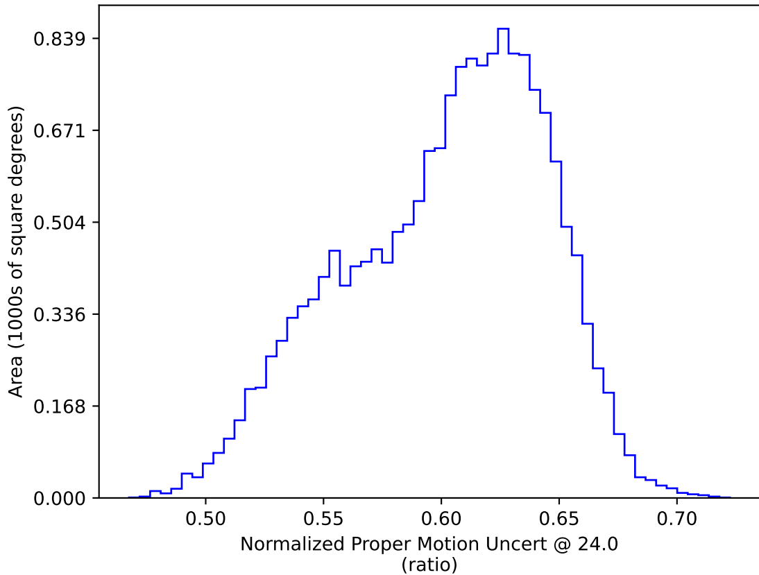
too_100_1v3.4_10yrs WFD: Normalized Proper Motion Uncert @ 24.0
