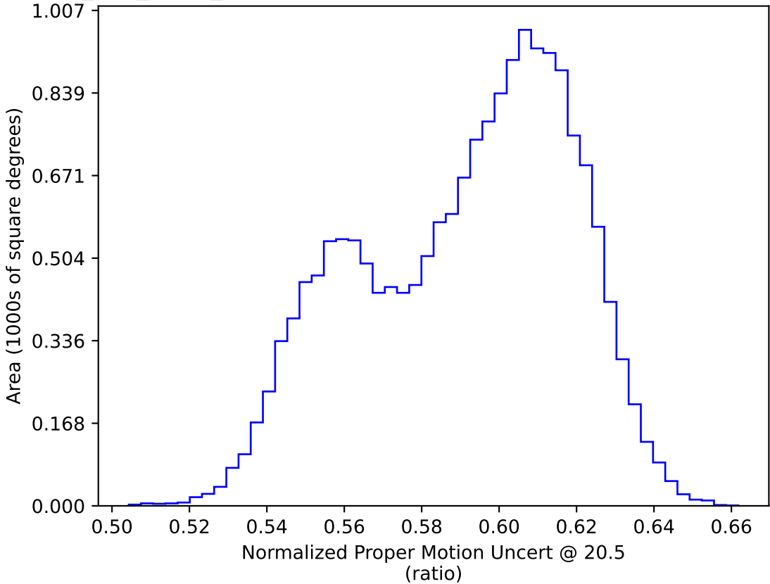
too_100_1v3.4_10yrs WFD: Normalized Proper Motion Uncert @ 20.5
