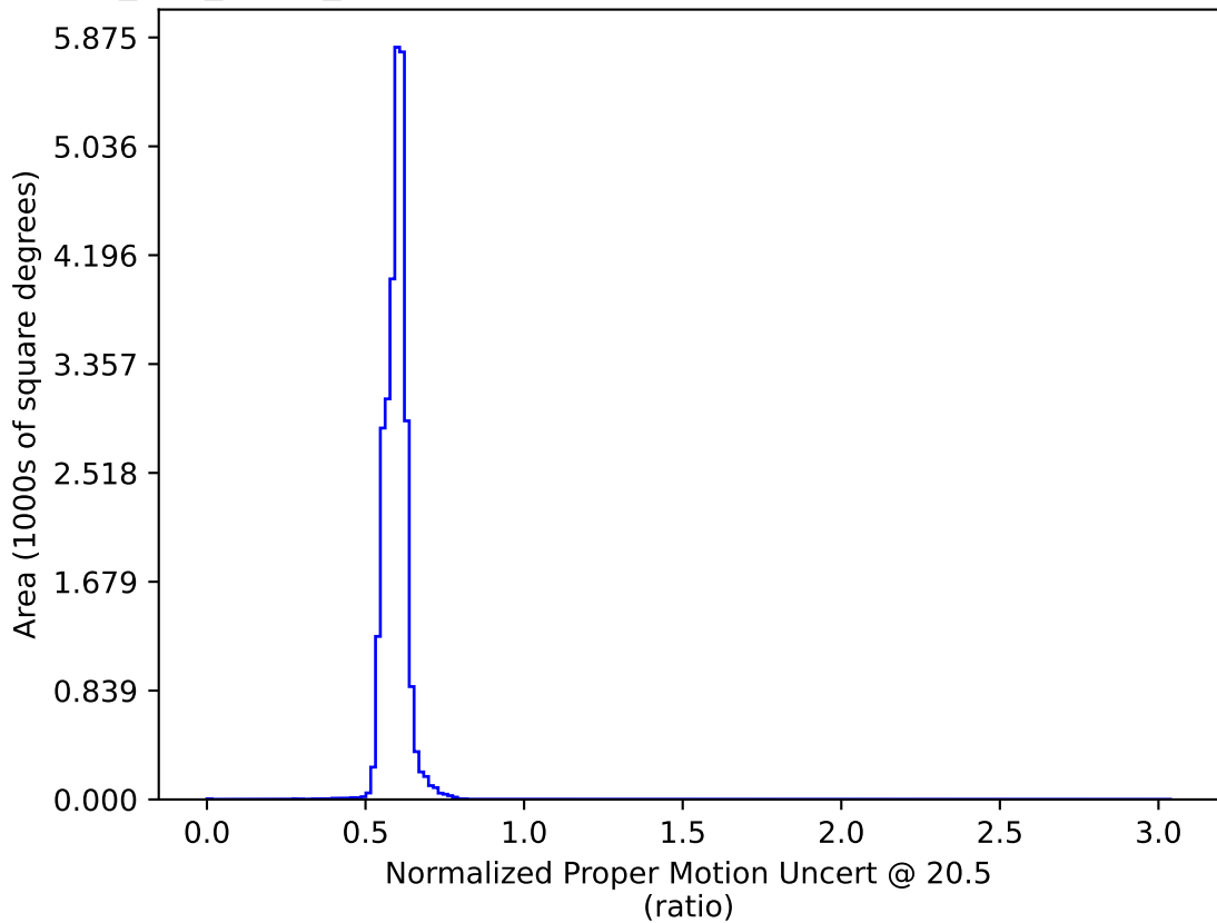
too_100_1v3.4_10yrs All sky: Normalized Proper Motion Uncert @ 20.5
