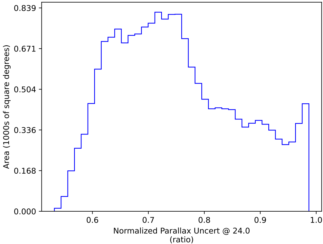
too_100_1v3.4_10yrs WFD: Normalized Parallax Uncert @ 24.0
