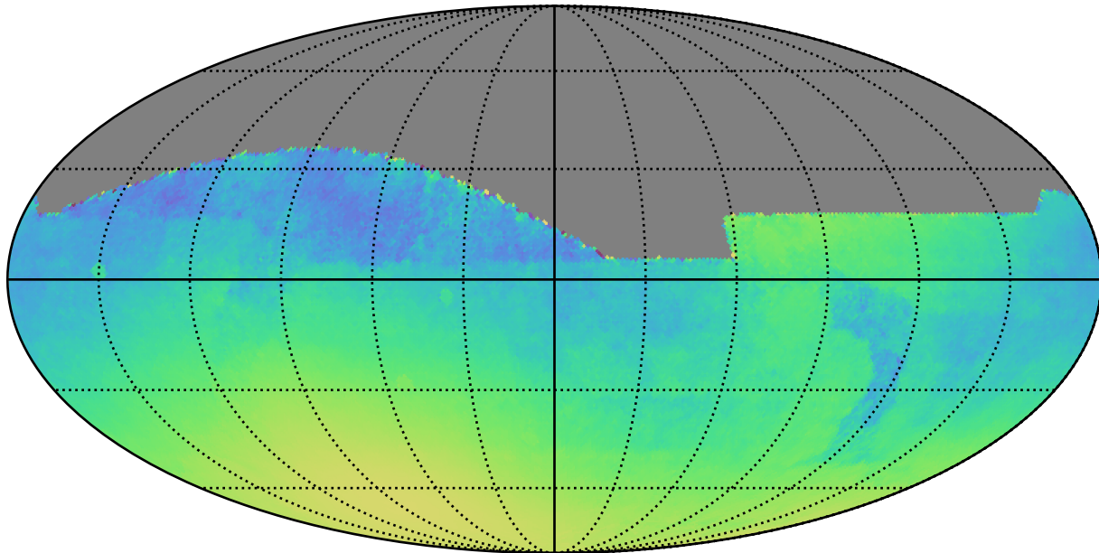
too_100_1v3.4_10yrs All sky: Normalized Parallax Uncert @ 24.0
