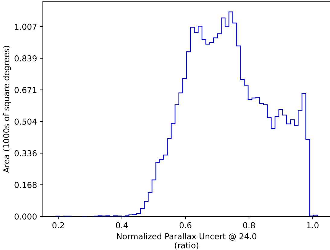
too_100_1v3.4_10yrs All sky: Normalized Parallax Uncert @ 24.0
