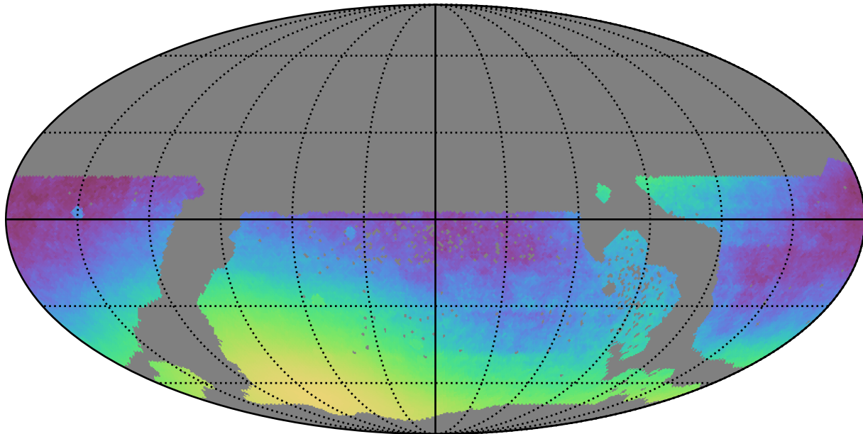
too_100_1v3.4_10yrs WFD: Normalized Parallax Uncert @ 22.4
