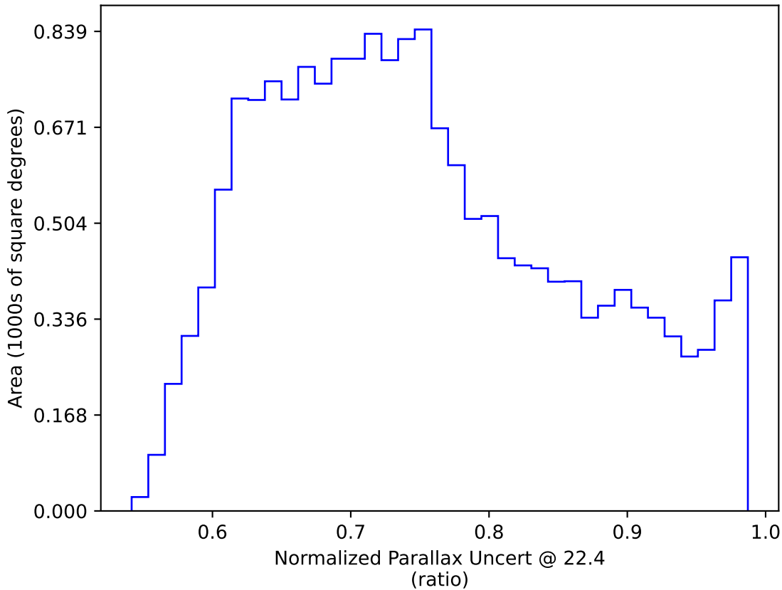
too_100_1v3.4_10yrs WFD: Normalized Parallax Uncert @ 22.4
