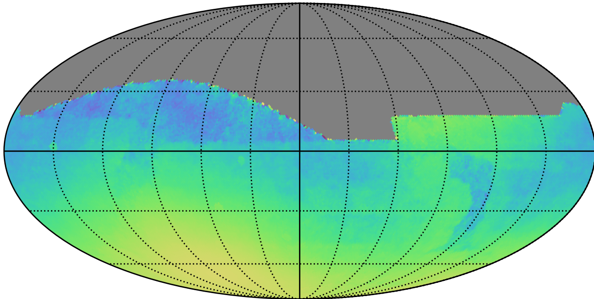
too_100_1v3.4_10yrs All sky: Normalized Parallax Uncert @ 22.4
