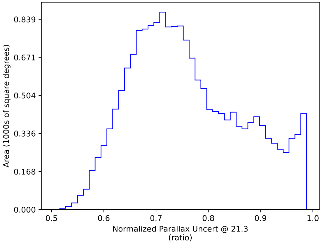
too_100_1v3.4_10yrs WFD y band only: Normalized Parallax Uncert @ 21.3
