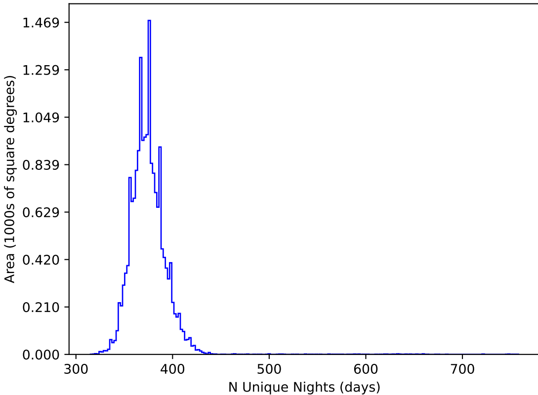
too_100_1v3.4_10yrs WFD all bands: N Unique Nights
