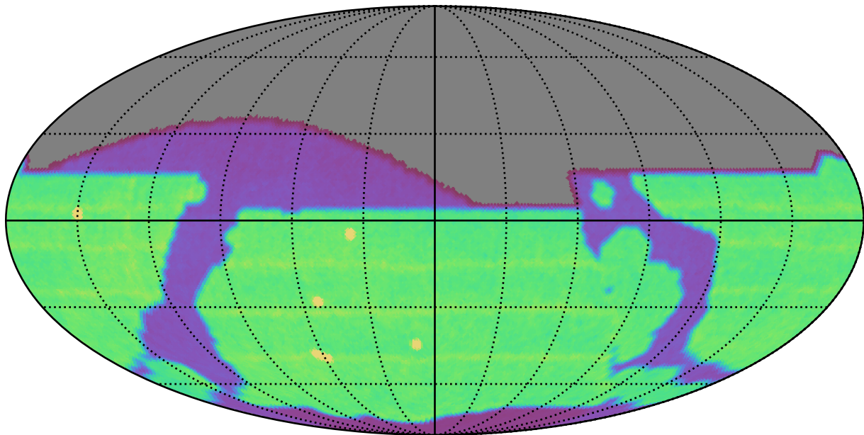
too_100_1v3.4_10yrs All sky all bands: N Unique Nights
