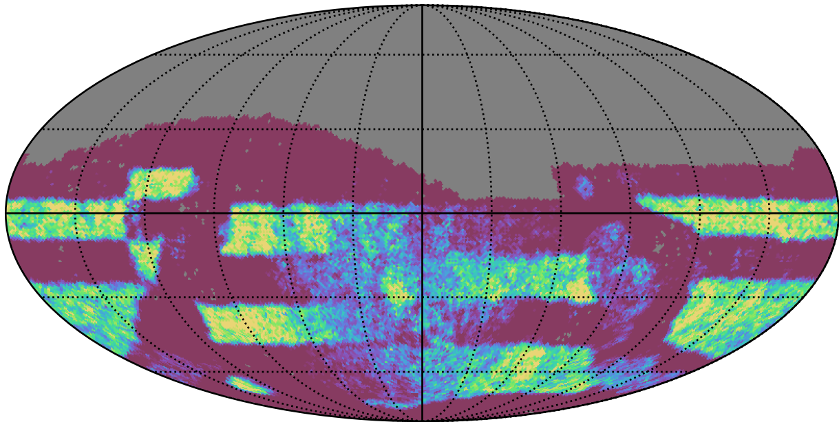
too_100_1v3.4_10yrs Yr 3-4 z band: NVisits
