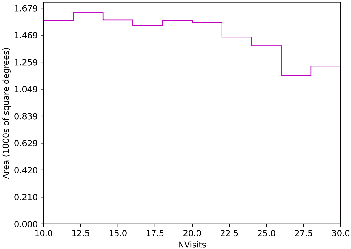
too_100_1v3.4_10yrs Yr 3-4 z band: NVisits
