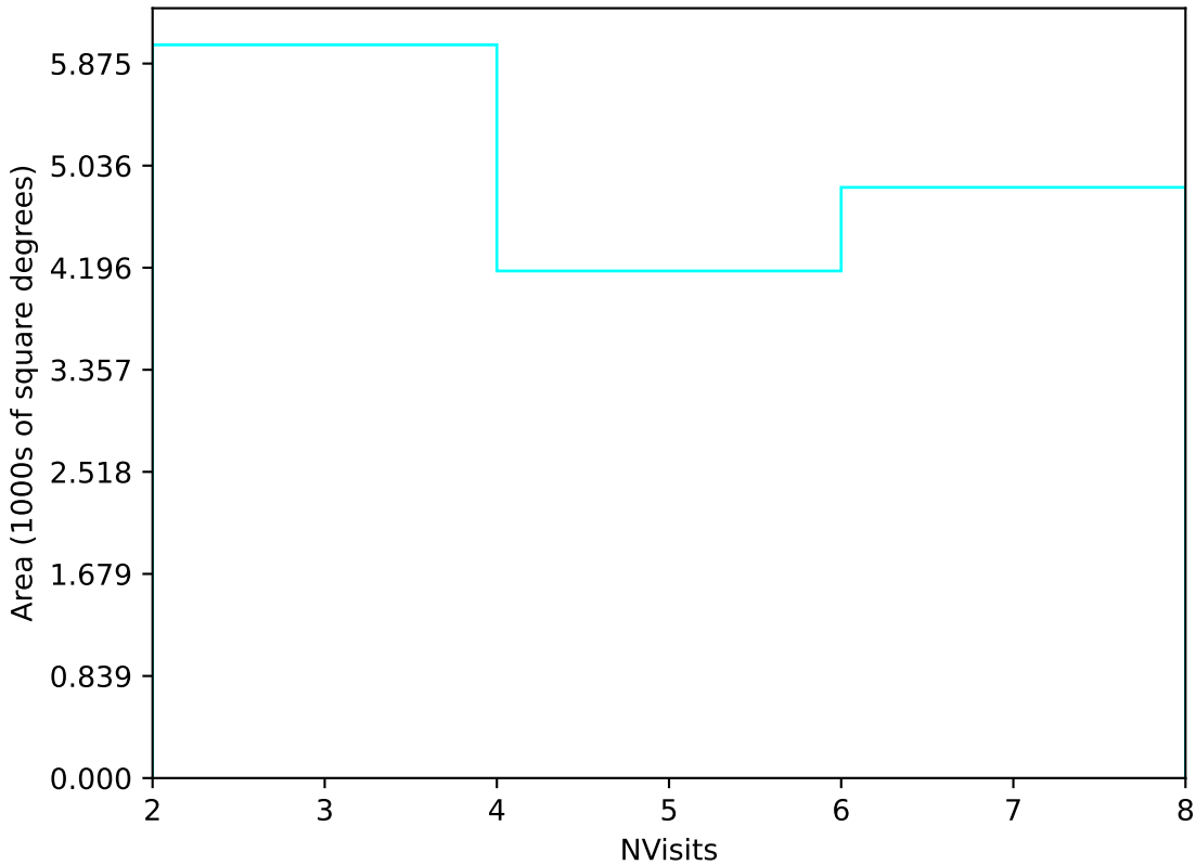
too_100_1v3.4_10yrs Yr 3-4 u band: NVisits
