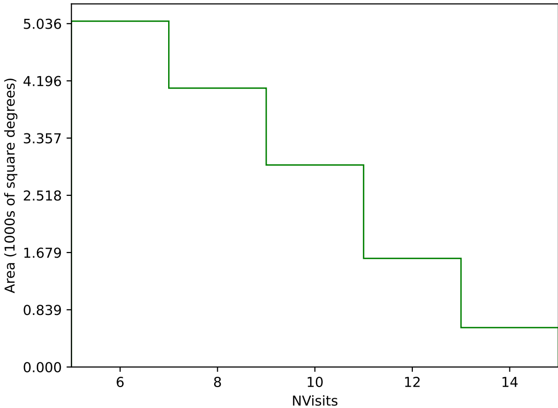
too_100_1v3.4_10yrs Yr 3-4 g band: NVisits
