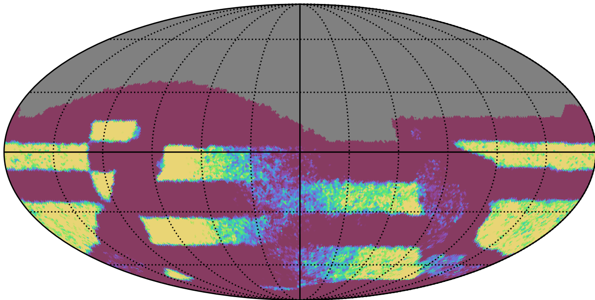
too_100_1v3.4_10yrs Yr 3-4 all bands: NVisits
