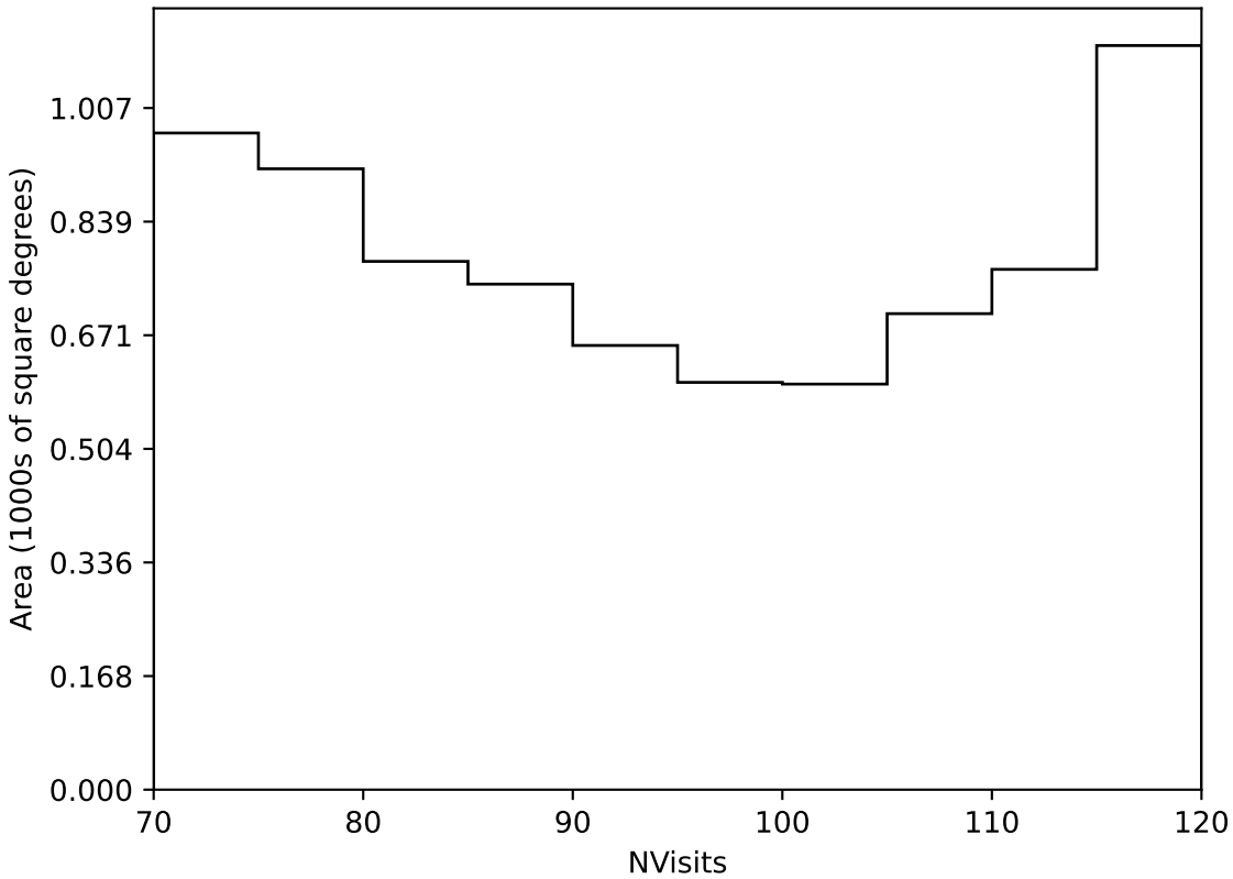
too_100_1v3.4_10yrs Yr 3-4 all bands: NVisits
