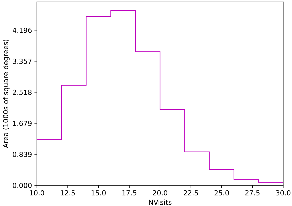
too_100_1v3.4_10yrs Yr 1 z band: NVisits
