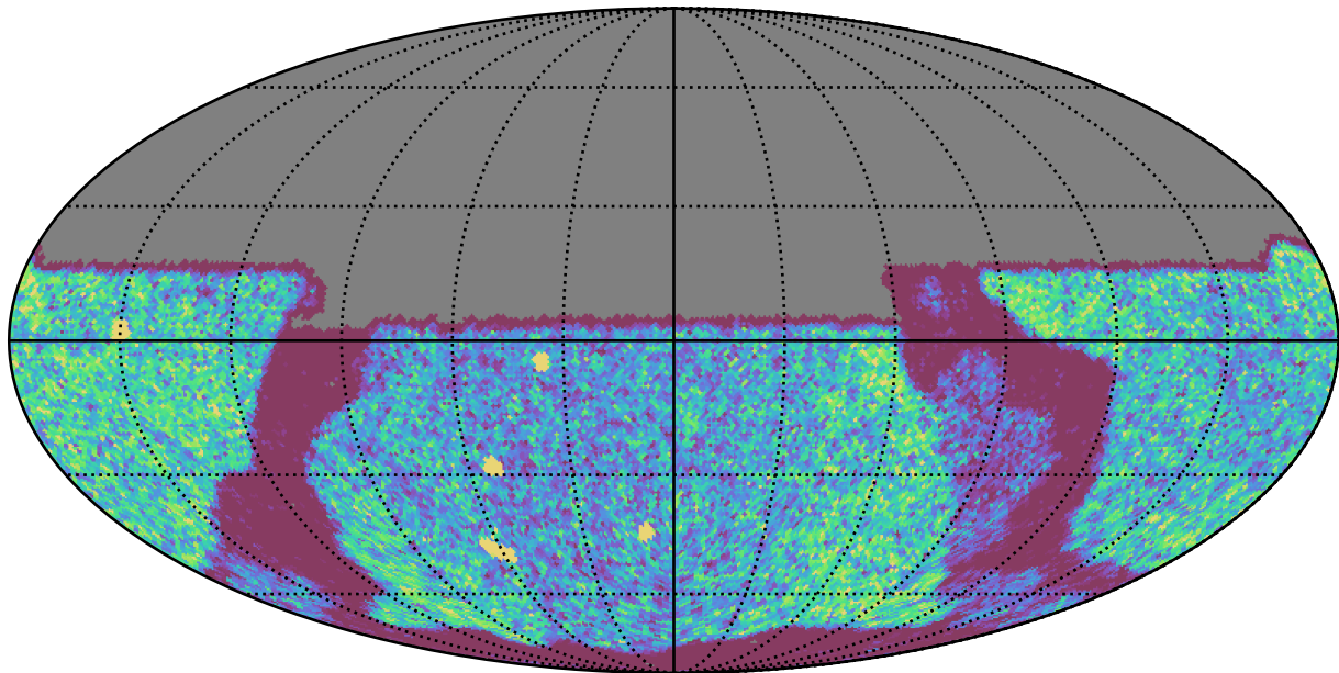
too_100_1v3.4_10yrs Yr 1 y band: NVisits
