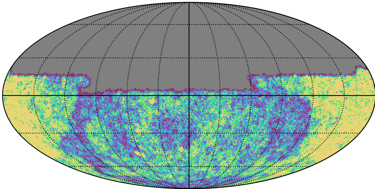
too_100_1v3.4_10yrs Yr 1 u band: NVisits
