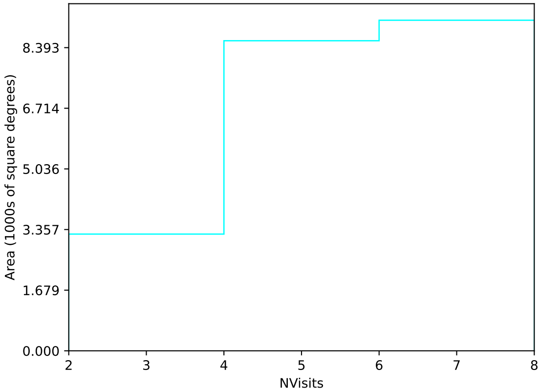
too_100_1v3.4_10yrs Yr 1 u band: NVisits
