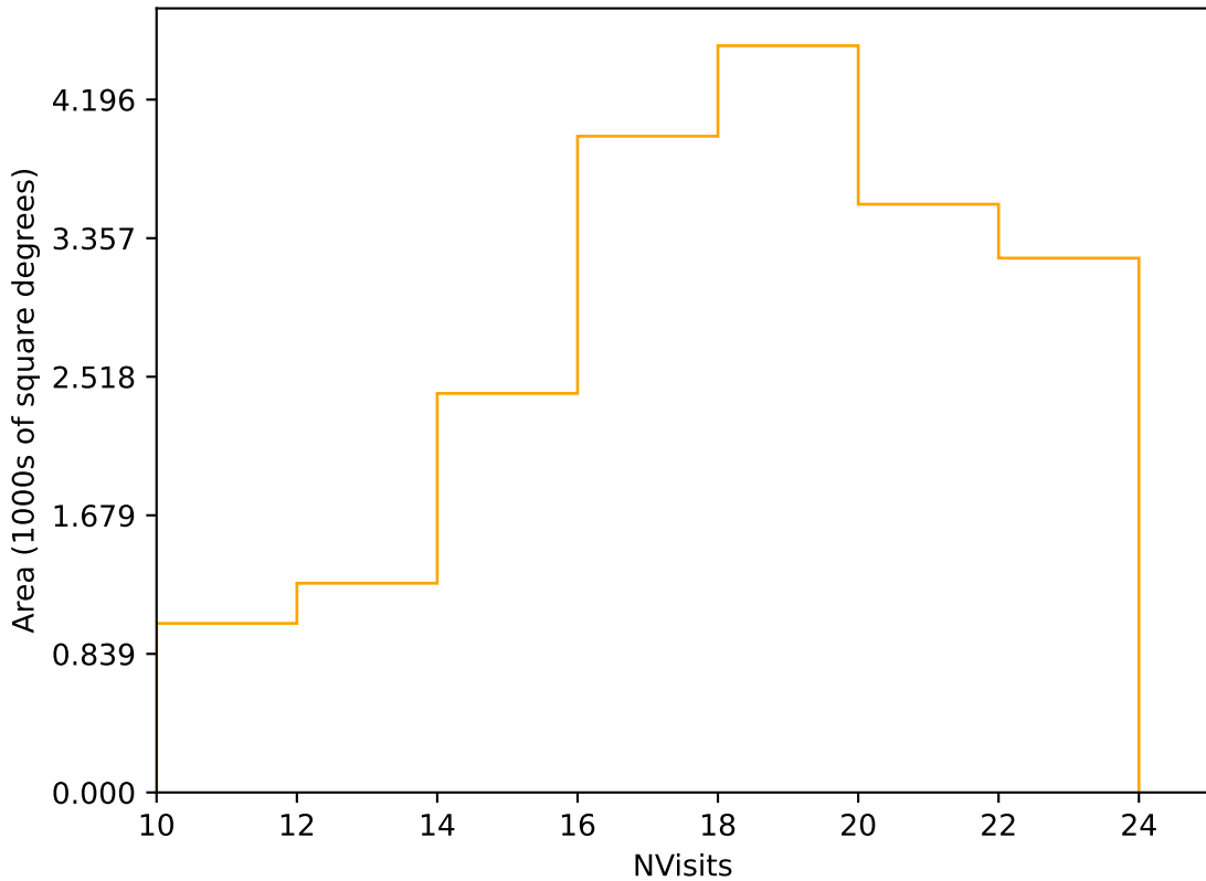
too_100_1v3.4_10yrs Yr 1 r band: NVisits
