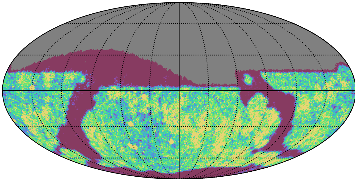
too_100_1v3.4_10yrs Yr 1 i band: NVisits
