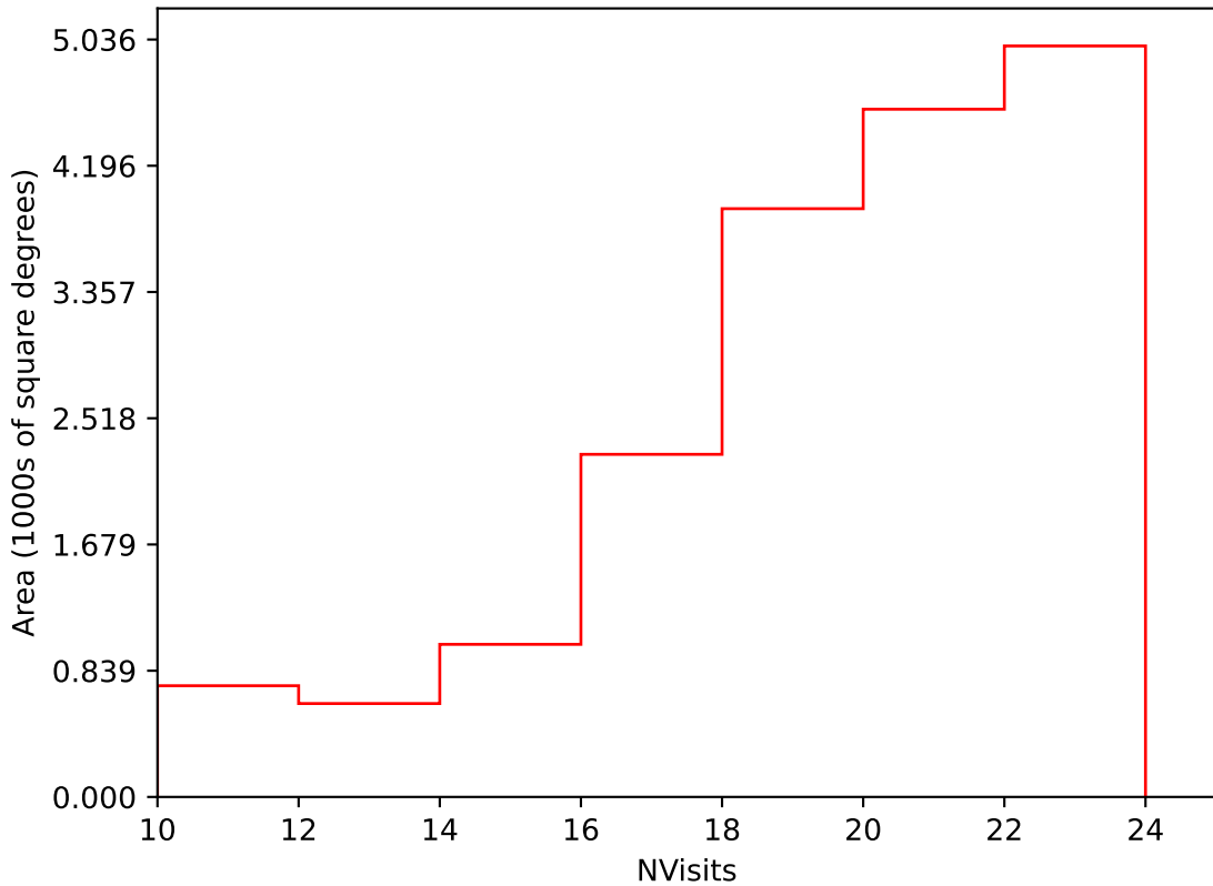
too_100_1v3.4_10yrs Yr 1 i band: NVisits
