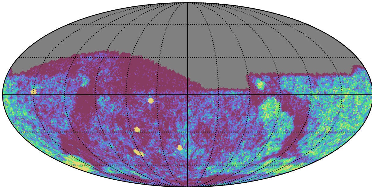
too_100_1v3.4_10yrs Yr 1 g band: NVisits
