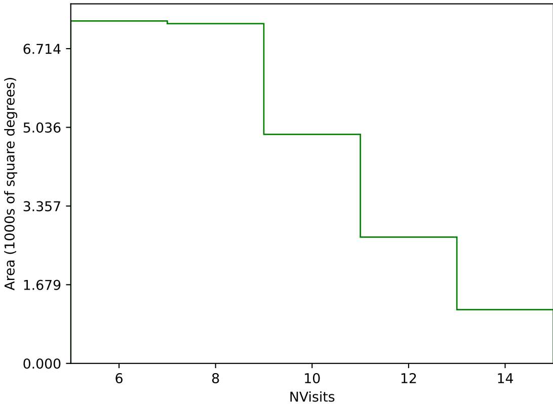
too_100_1v3.4_10yrs Yr 1 g band: NVisits
