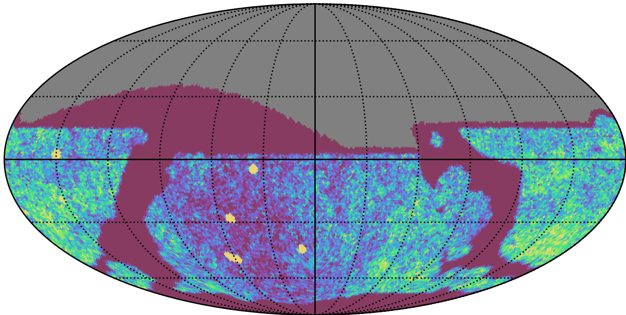
too_100_1v3.4_10yrs Yr 1 all bands: NVisits
