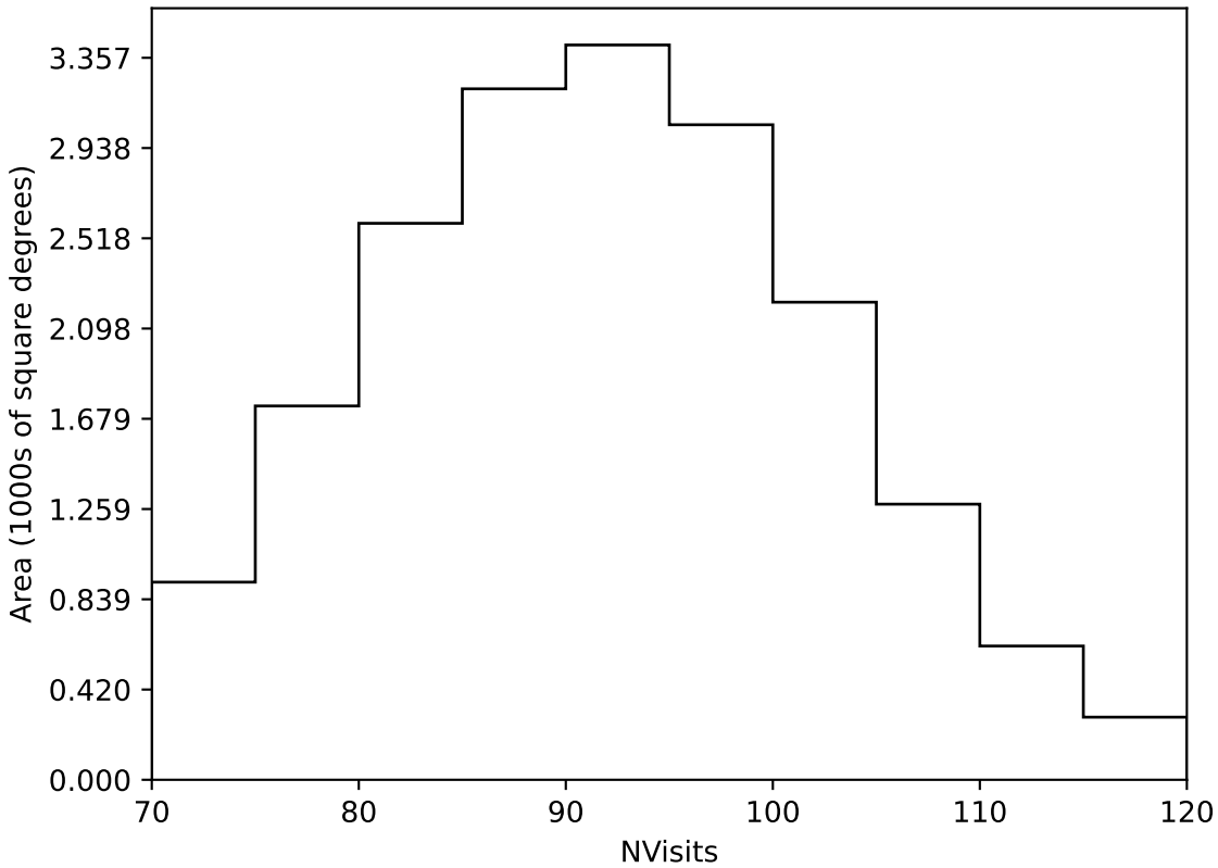
too_100_1v3.4_10yrs Yr 1 all bands: NVisits
