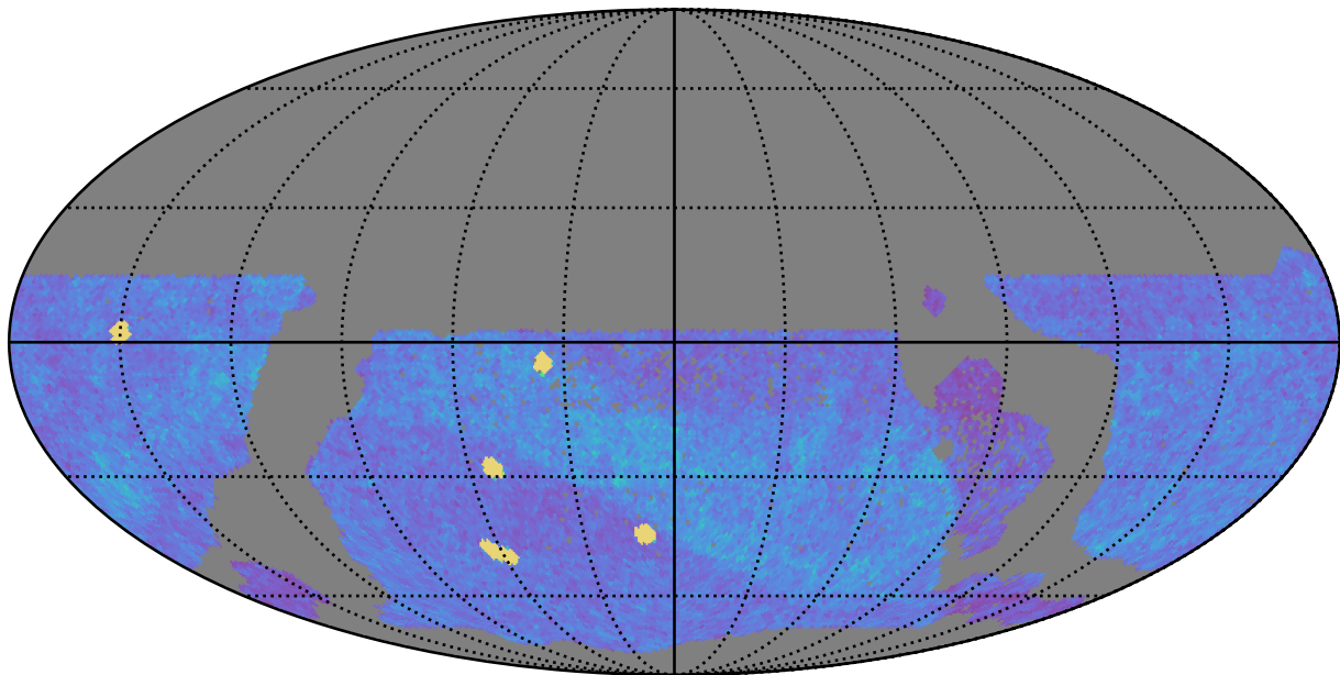
too_100_1v3.4_10yrs WFD z band: NVisits
