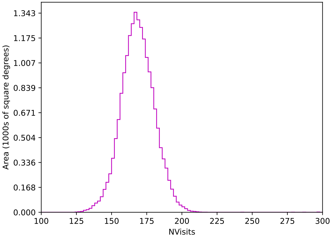
too_100_1v3.4_10yrs WFD z band: NVisits
