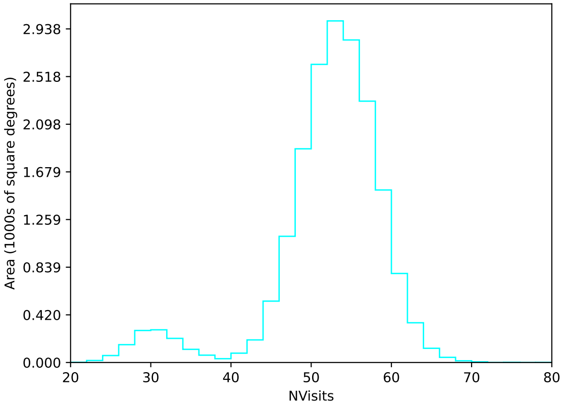
too_100_1v3.4_10yrs WFD u band: NVisits
