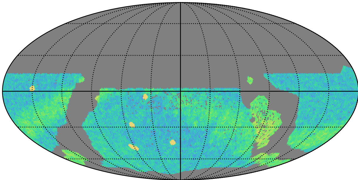
too_100_1v3.4_10yrs WFD r band: NVisits
