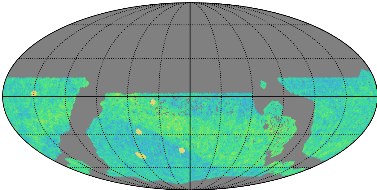
too_100_1v3.4_10yrs WFD i band: NVisits
