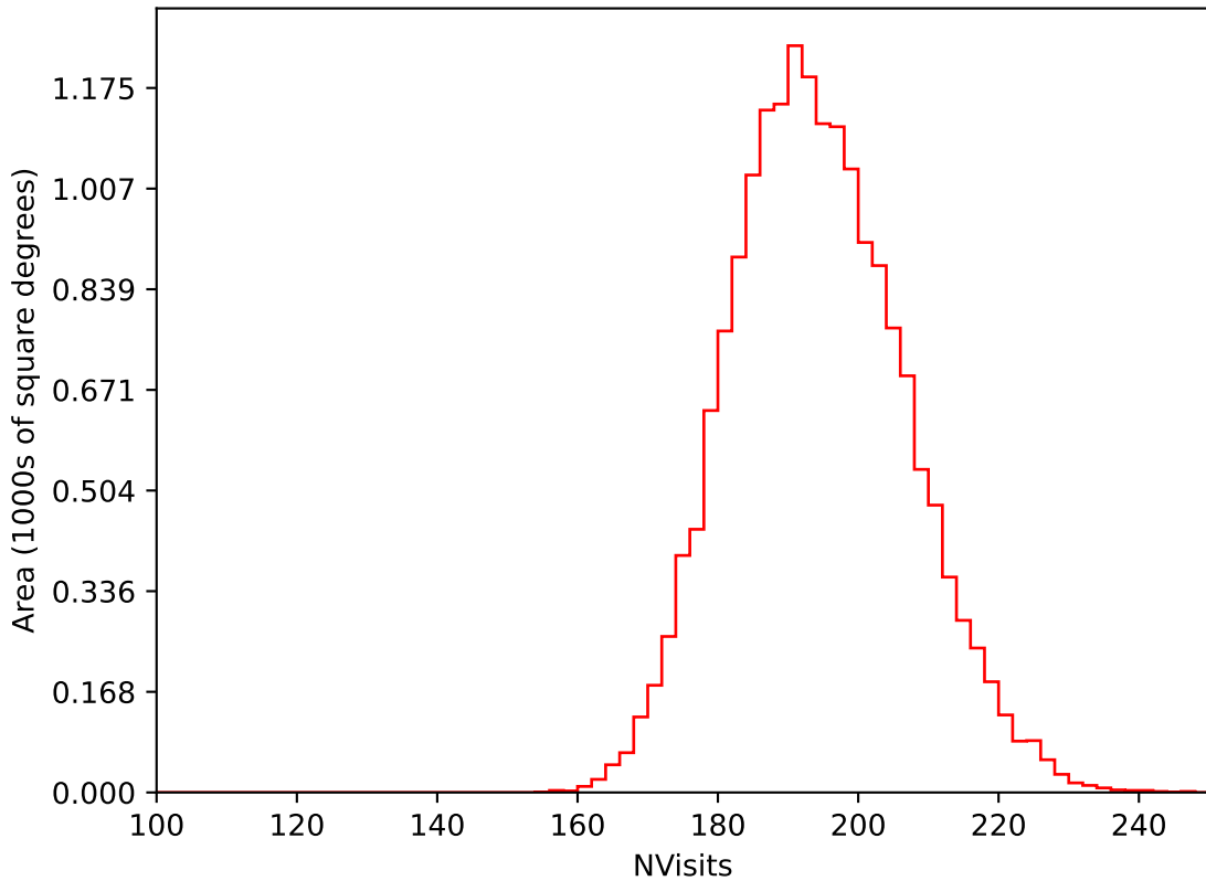
too_100_1v3.4_10yrs WFD i band: NVisits
