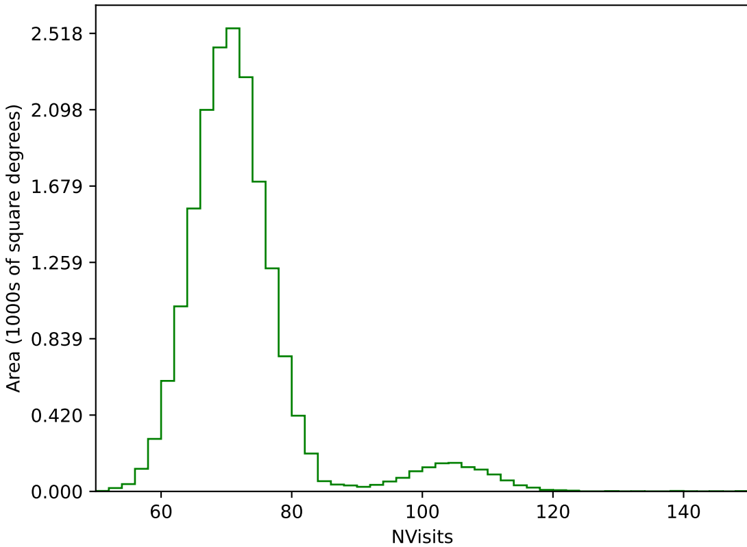
too_100_1v3.4_10yrs WFD g band: NVisits
