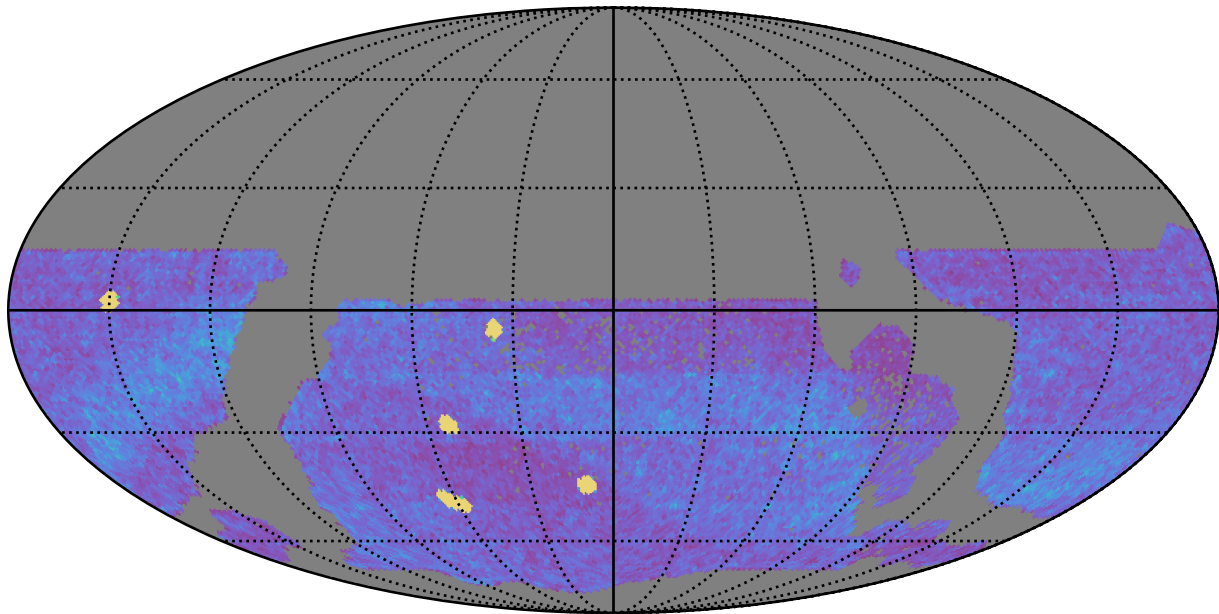
too_100_1v3.4_10yrs WFD all bands: NVisits
