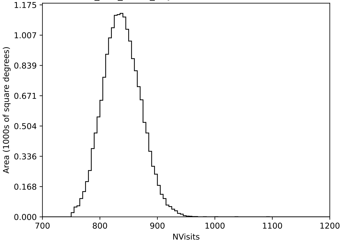
too_100_1v3.4_10yrs WFD all bands: NVisits
